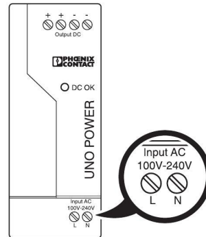
Figure 10 Screw connection for input AC L/N
